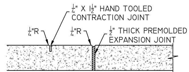
TYPICAL CONTRACTION & EXPANSION JOINTS
