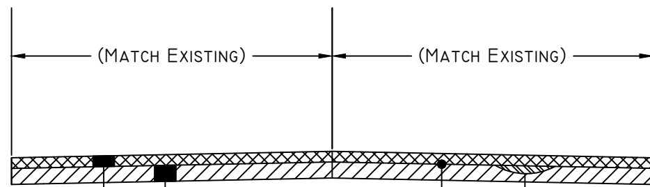
TYPICAL SECTION (SHADY LANE, MIDWAY STREET, WILSON COURT, MCINTYRE AVENUE, GUY STREET, & CENTER STREET)
