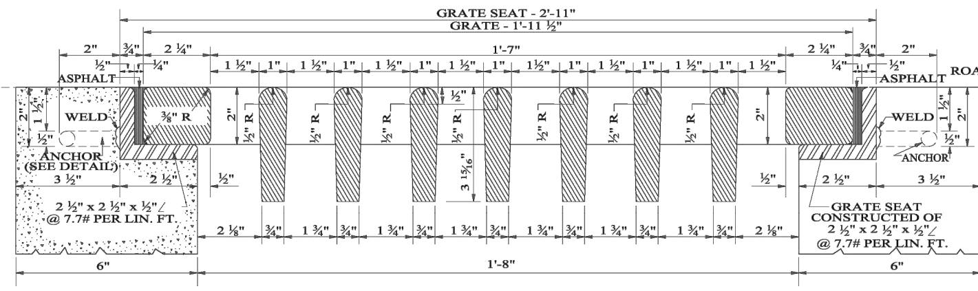
SECTION "BB" (THROUGH GRATE)
