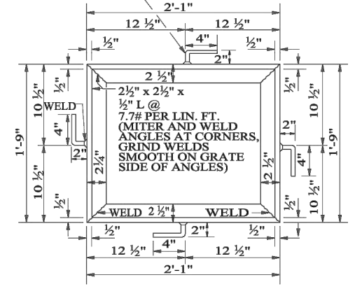
PLAN VIEW OF GRATE SEAT
