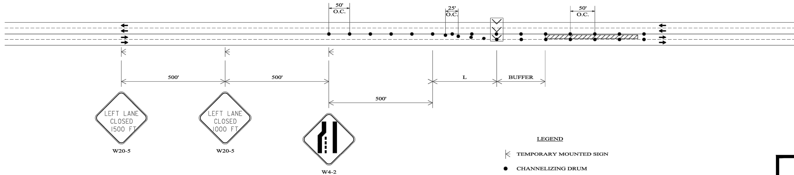
TYPICAL SCHEME FOR INSIDE LANE CLOSURE
