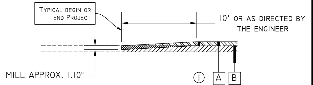
TYPICAL BEGIN/END PROJECT IN OVERLAY SECTIONS
