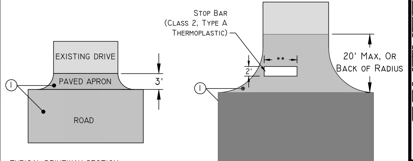
TYPICAL DRIVEWAY SECTION
