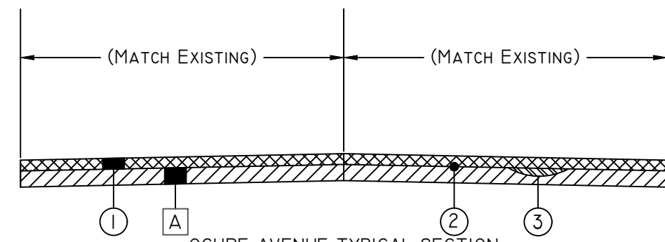
OCHRE AVENUE TYPICAL SECTION STA 3+65.68 - STA 8+47.52
