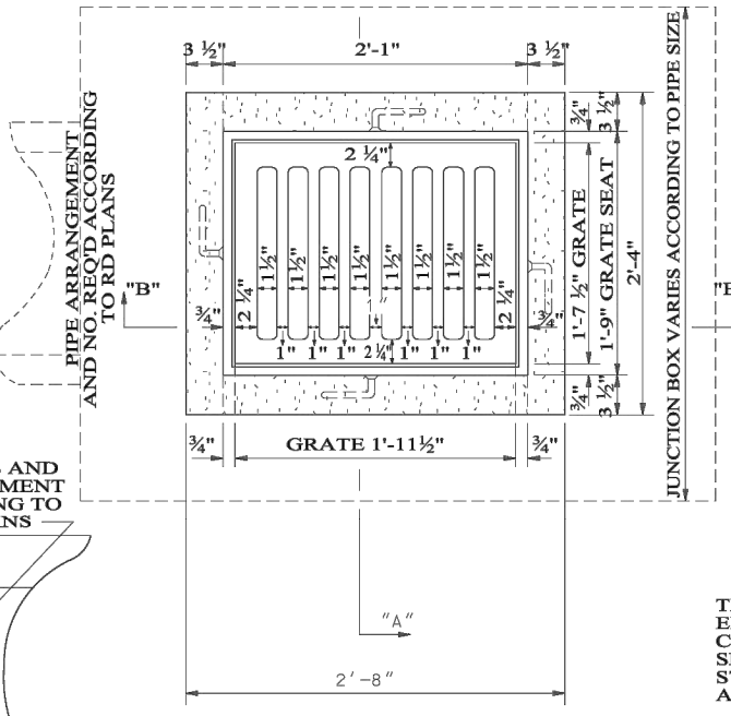
PLAN VIEW OF INLET AND GRATE DUCTILE OR MALLEABLE IRON GRATE CASTING
