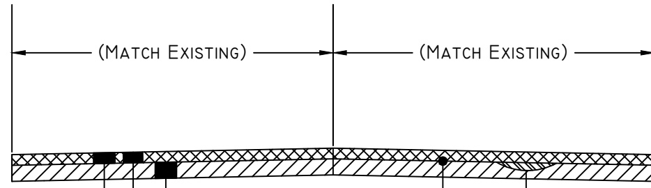
TYPICAL SECTION (STANLEY DRIVE, ODOM DRIVE, EAST STATE STREET, MIDDLE STREET, WEST ROSE STREET, & GRIFFIN STREET)
