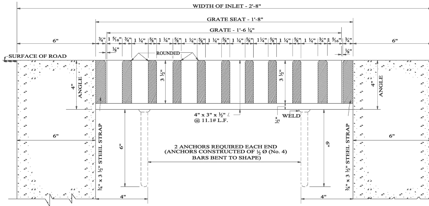
ENLARGED SECTION "AA"
