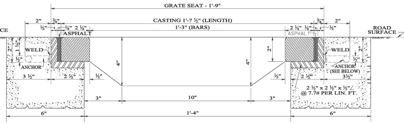
SECTION "AA" (THROUGH GRATE)
