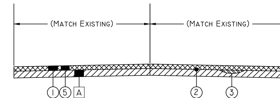
OCHRE AVENUE TYPICAL SECTION STA 8+47.52 - STA 11+88.98
