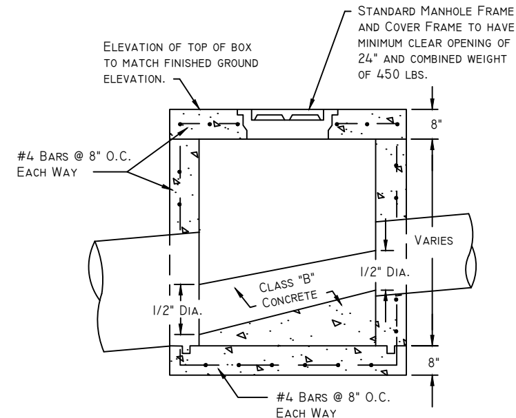
JUNCTION BOX DETAIL NOT TO SCALE
