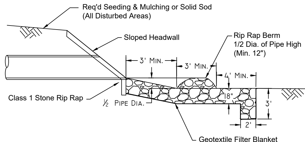
Typical Slope Paved Headwall Rip Rap Pipe Discharge Outlet Energy Dissipator Not to Scale
