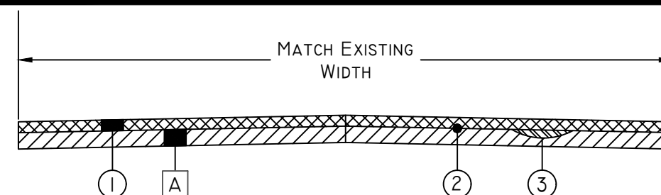
TYPICAL SECTION (MAIN STREET)
