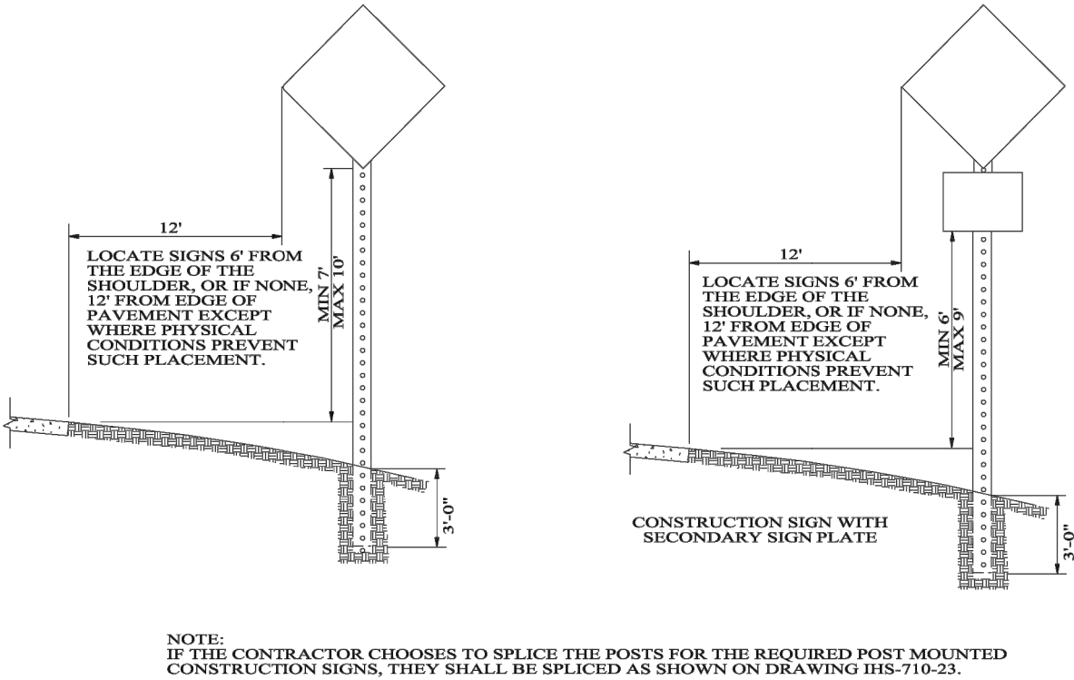
HEIGHT AND LATERAL LOCATION OF POST MOUNTED CONSTRUCTION SIGNS
