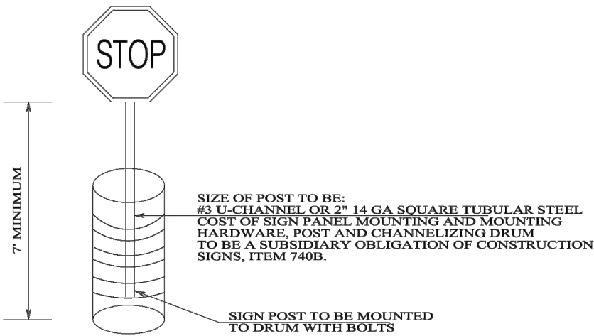
DETAIL FOR DRUM MOUNTED CONSTRUCTION SIGNS
