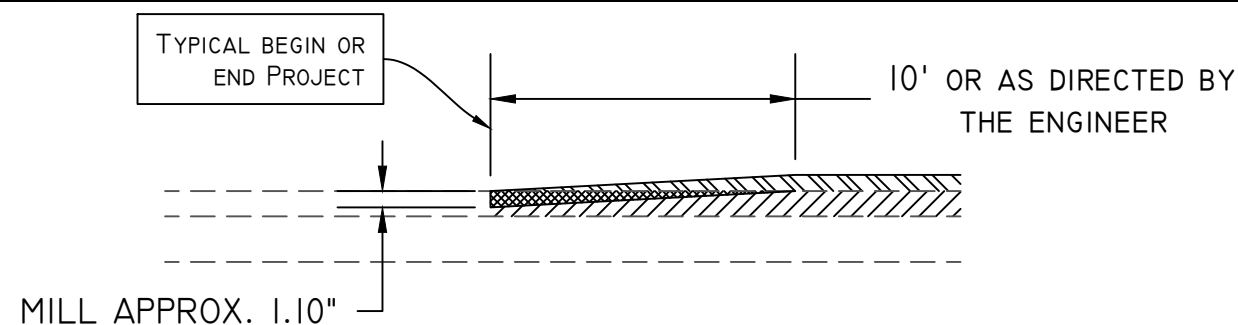
TYPICAL BEGIN/END PROJECT IN OVERLAY SECTIONS
