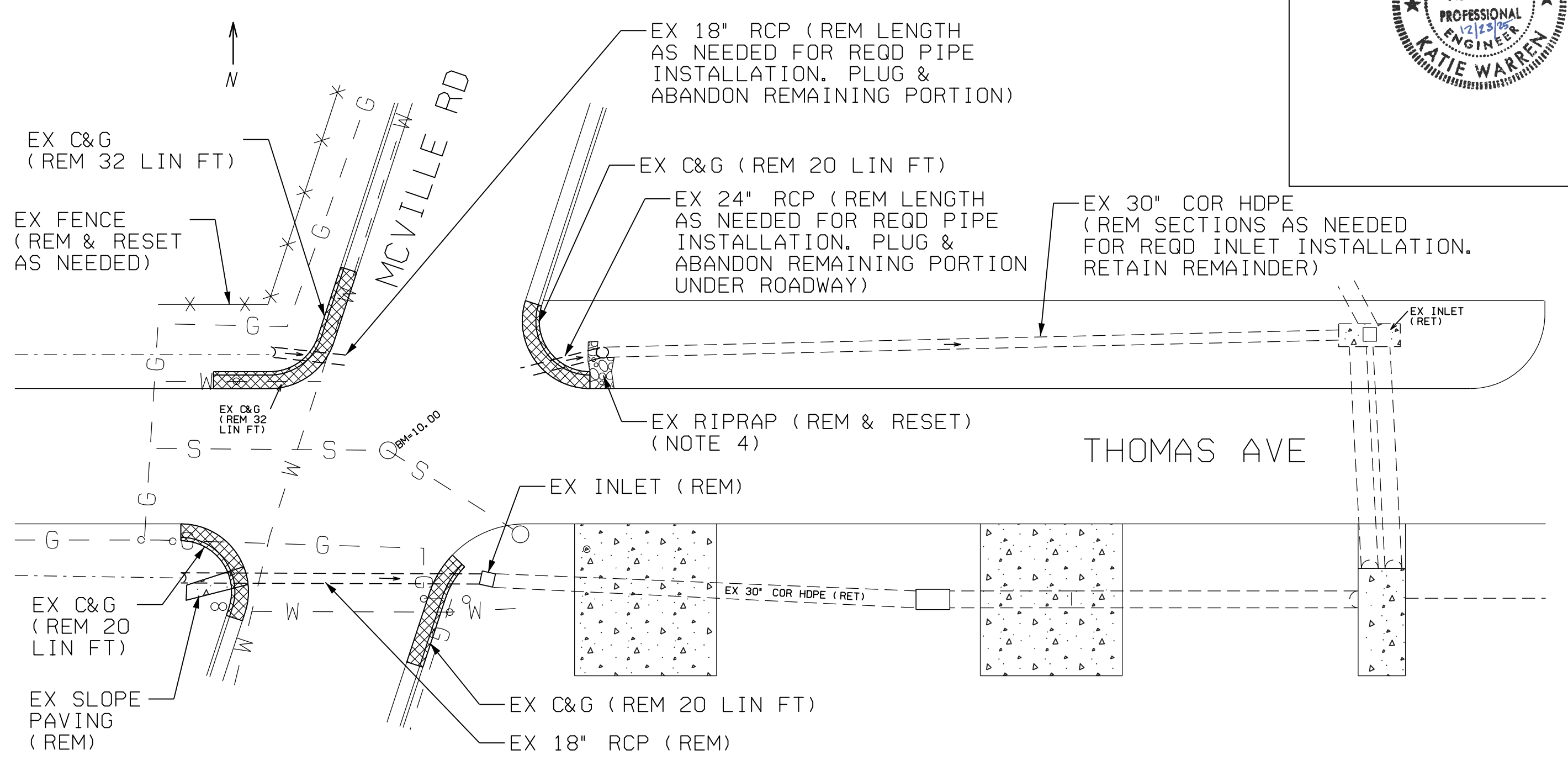
DEMOLITION PLAN
