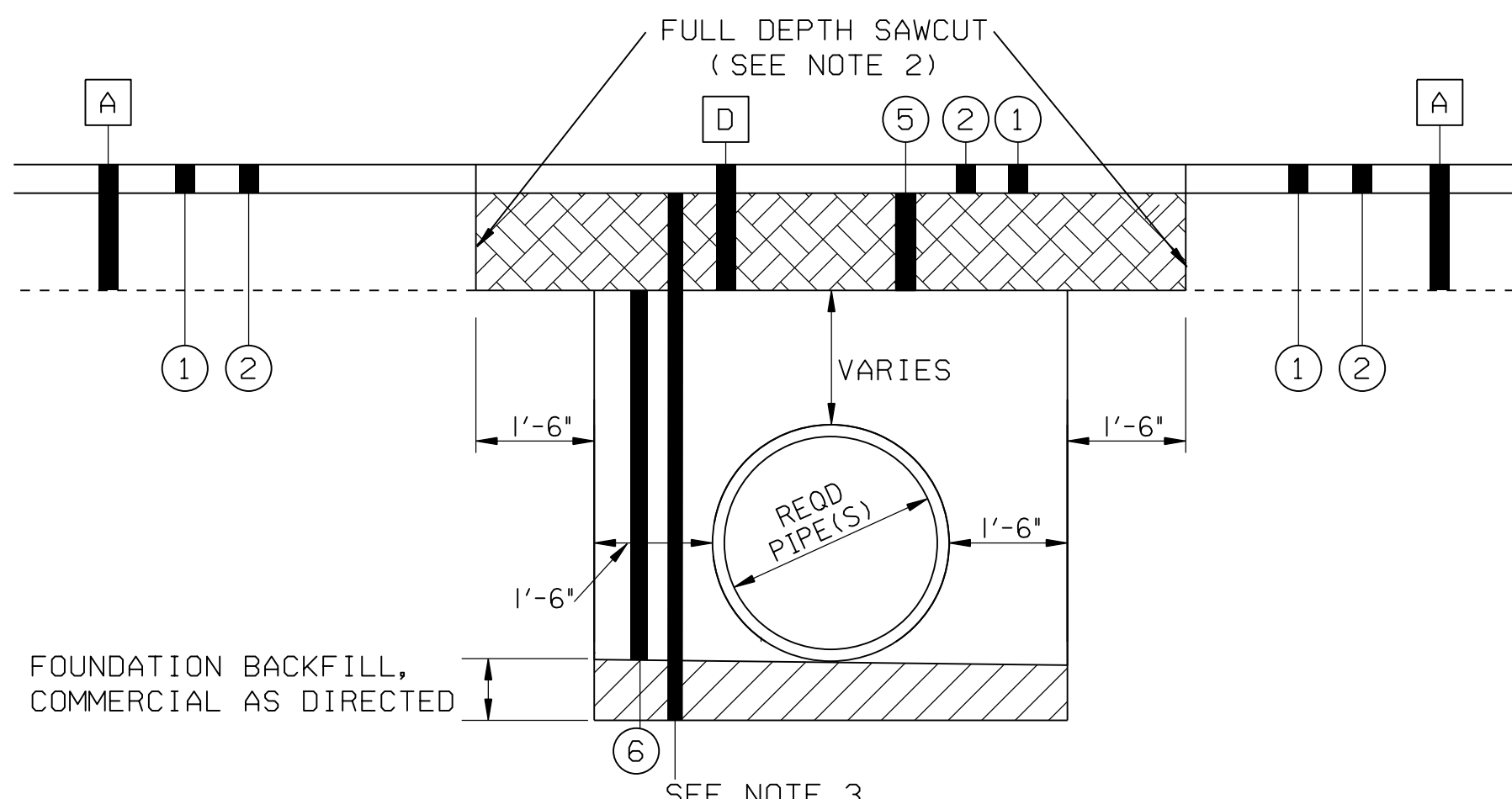
ASPHALT PAVEMENT DETAIL OPEN-CUT FOR REQD ROADWAY PIPE
