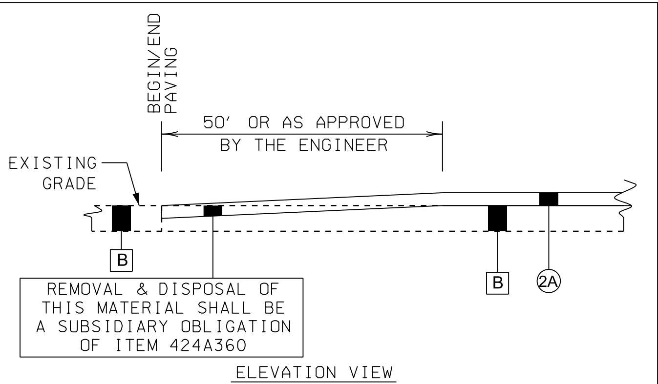
ELEVATION VIEW
