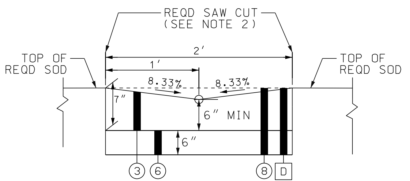
CONC GUTTER DETAIL
