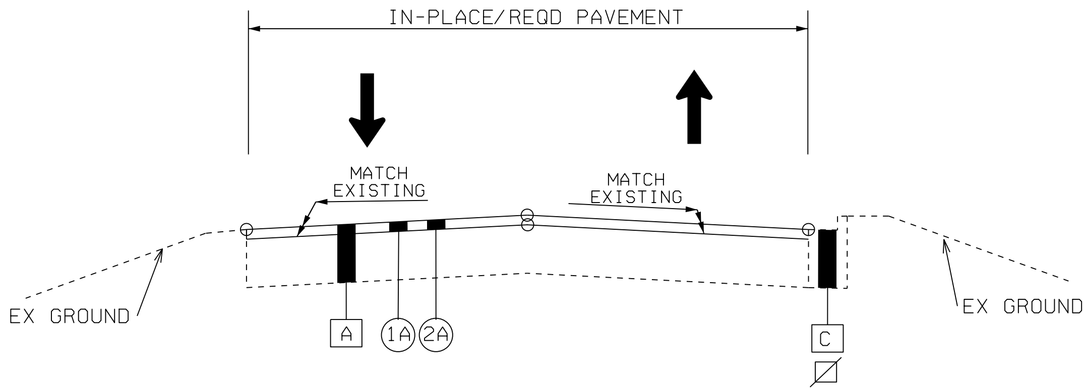
TYPICAL SECTION III ▲ 1.25" MILL & OVERLAY
