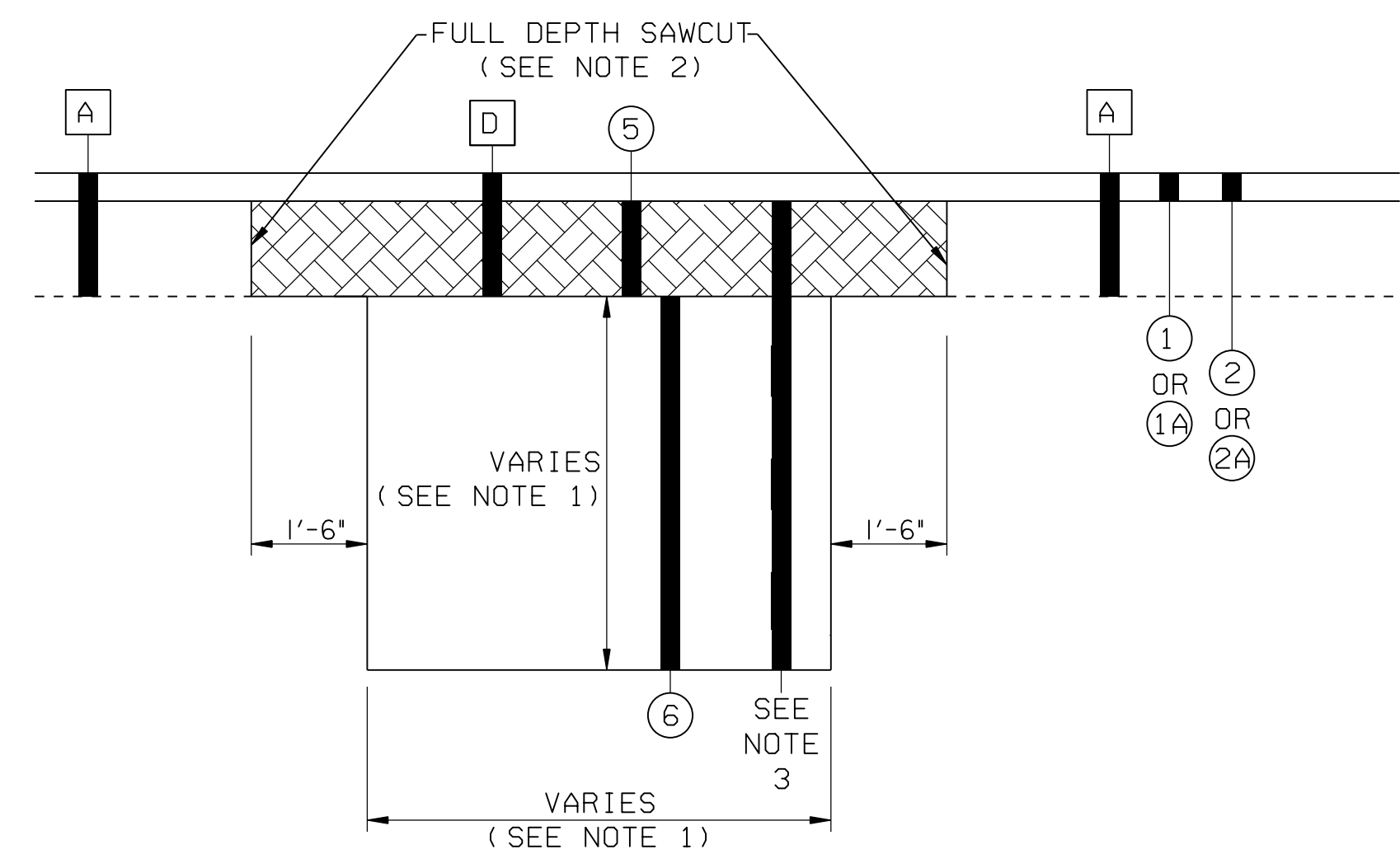
ASPHALT PATCHING DETAIL
