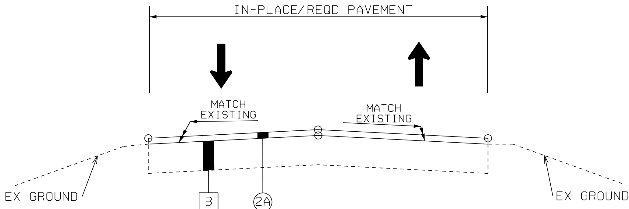
TYPICAL SECTION IV ● 1.25" OVERLAY
